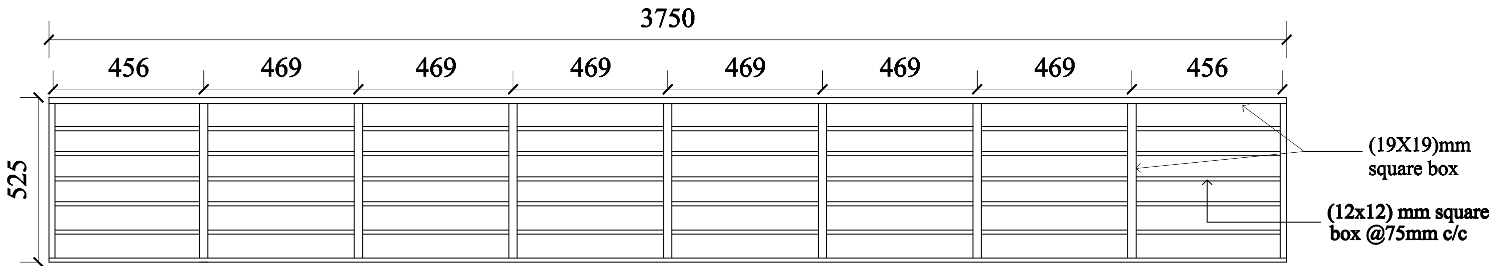
FRONT VIEW
