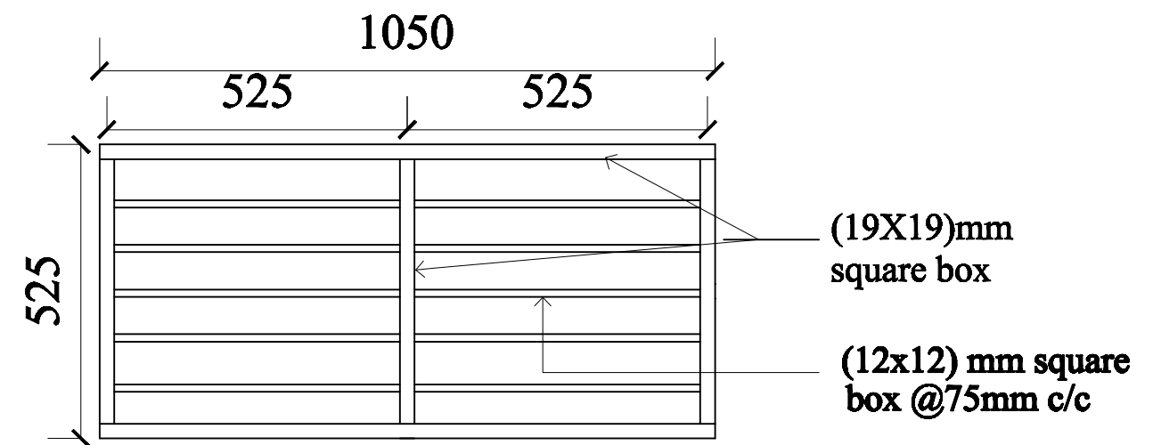
SIDE VIEW
